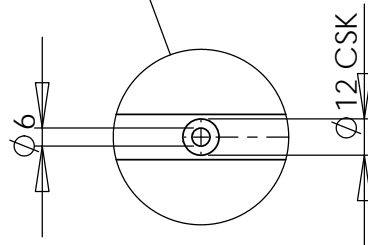
DETAIL E SCALE 2 : 5
